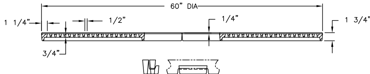
INTERLOCK ASSEMBLY DETAIL
